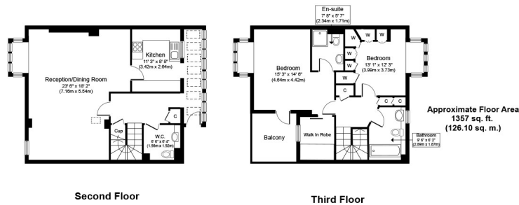
Third Floor
